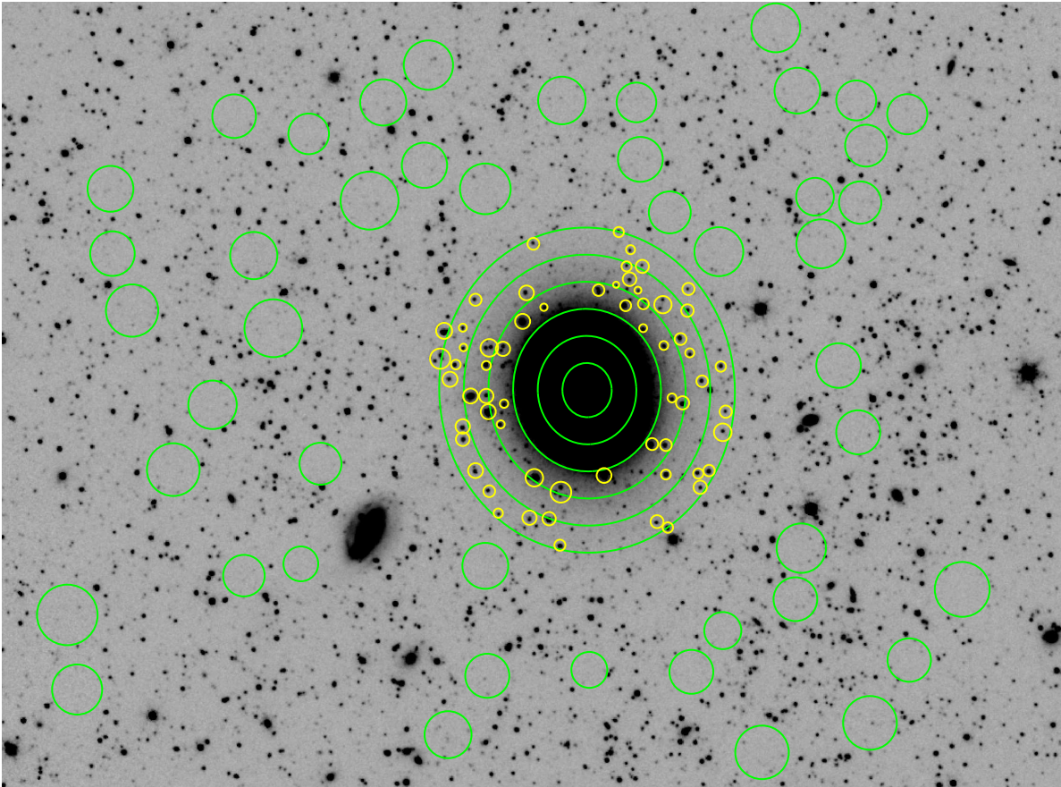
Fig. 2.— A 16'.5 \times 9'.7 portion of the Spitzer 3.6 \mu\text{m} mosaic of NGC 5273. The ellipses demonstrate the annular regions for extracting photometry and the large and small circles respectively show the sky apertures and foreground star masks. North is up, East is to the left.
