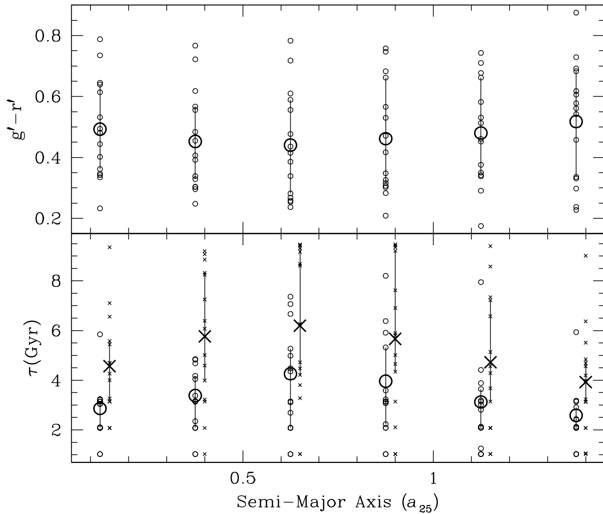
Fig. 6.— The distribution of g' - r' and \tau parameters. The large symbols indicate the average value for each radius; in the bottom panel the circles stem from a delayed star formation history and the (slightly offset for clarity) crosses indicate the single exponential star formation history model. The vertical lines mark the 25 th –75 th quartile spreads.
