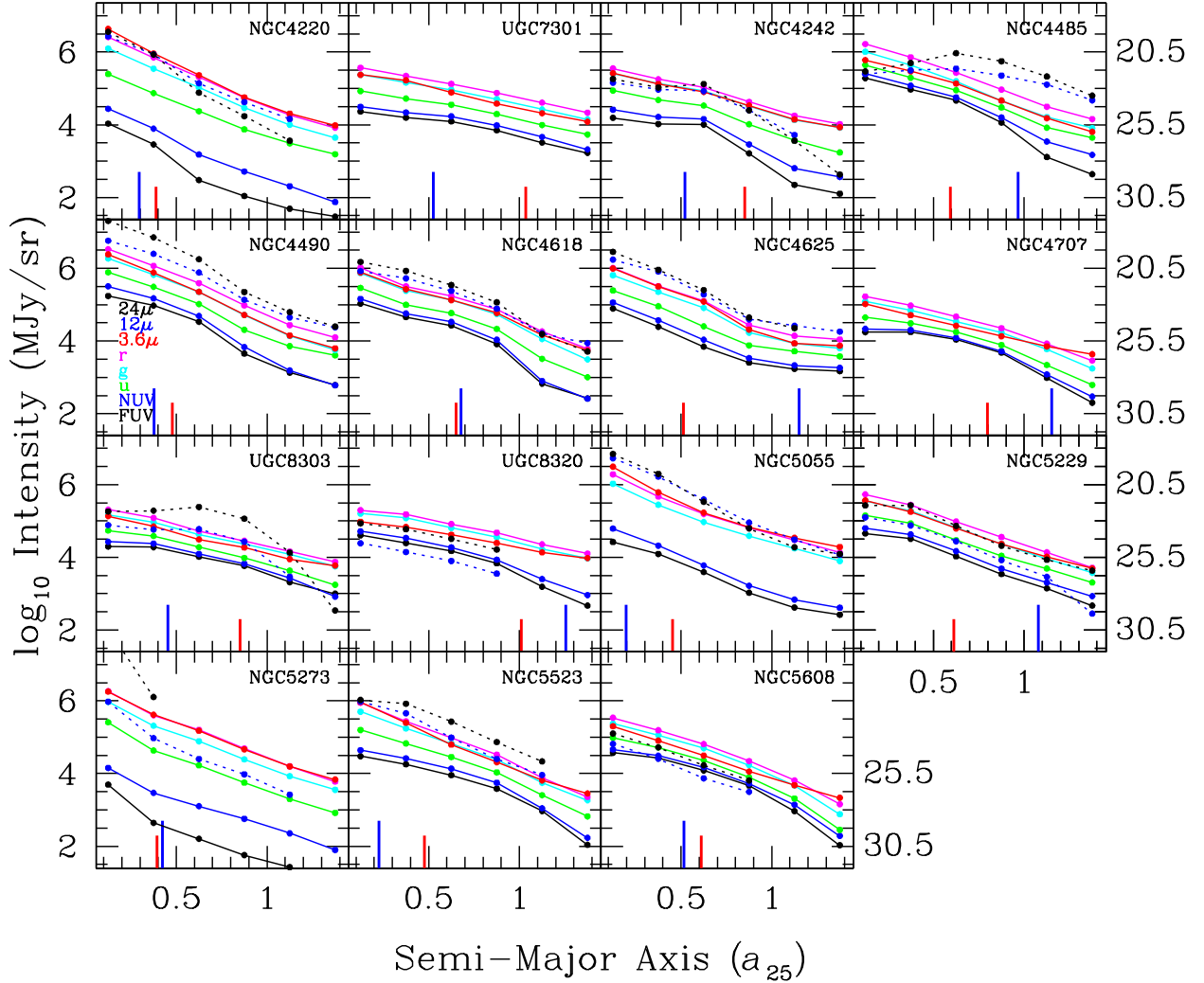
Fig. 4.— The observed multi-wavelength surface brightness profiles corrected for foreground Milky Way dust attenuation. The right-hand axis is AB mag arcsec -2 . The dotted curves are for dust emission, and the vertical blue (red) lines near the bottom of each panel indicate 3 kpc (twice the r' half-light radius).
