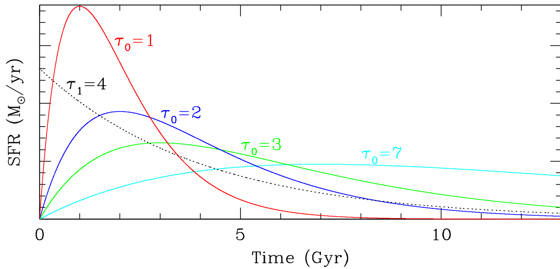
Fig. 3.— Four examples of a “delayed” star formation history along with an example of a decreasing exponential star formation history (dotted curve). All values shown are in Gyr.
