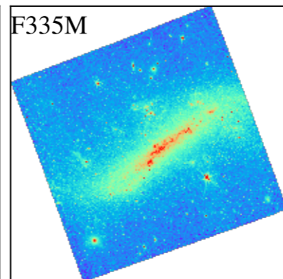
NGC4731
