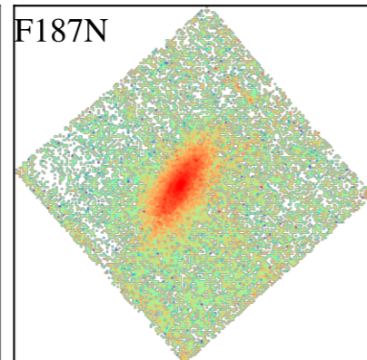
NGC1546
