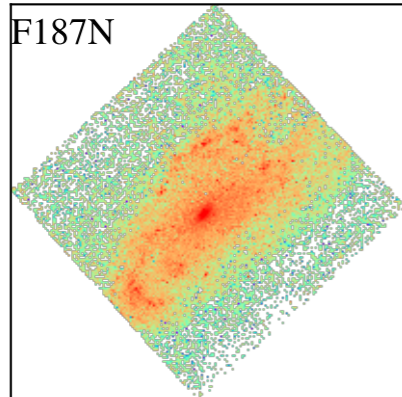
NGC1792
