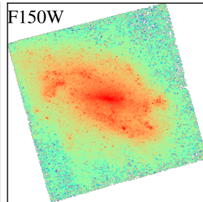
NGC1559
