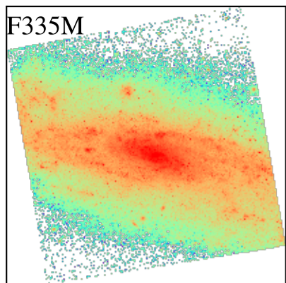
NGC3511
