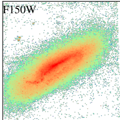
NGC1511
