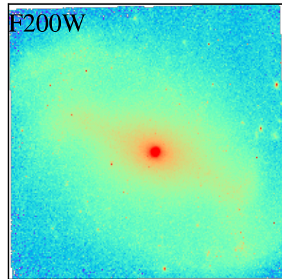
NGC2566
