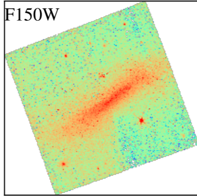
NGC4731
