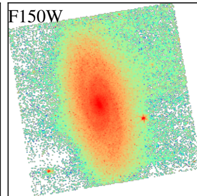
NGC2090
