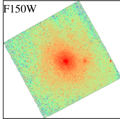
NGC4571
