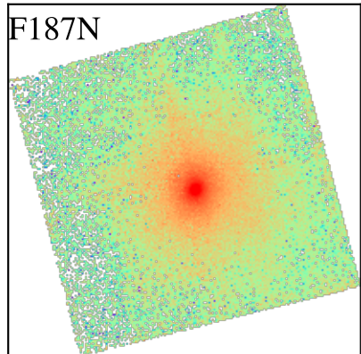
NGC2775
