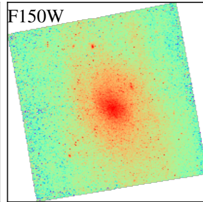
NGC5042
