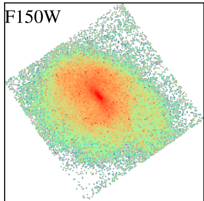
IC5273
