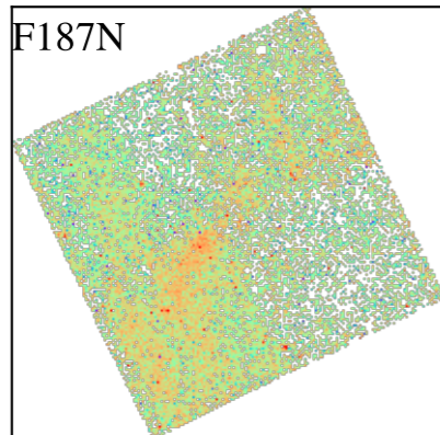
NGC1809
