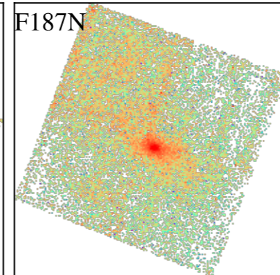
NGC1637
