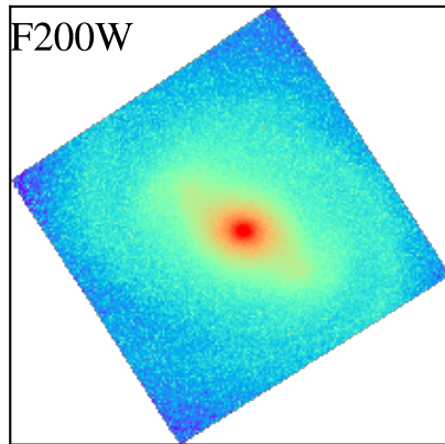
NGC4579
