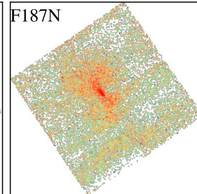
IC5273
