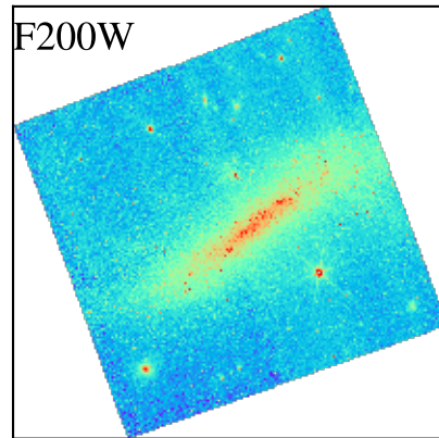
NGC4731
