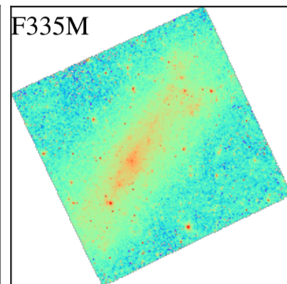
NGC1809
