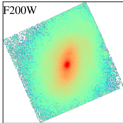
NGC3626
