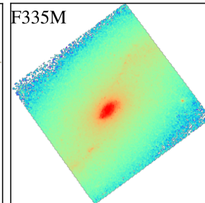
NGC1808
