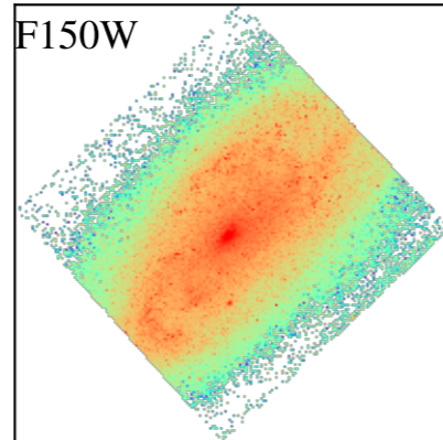
NGC1792
