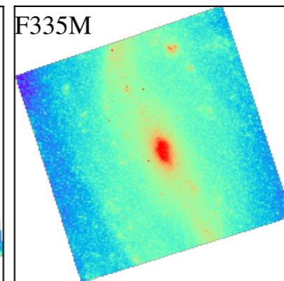
NGC2903
