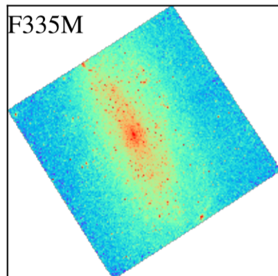
NGC7456
