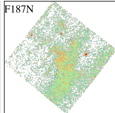
NGC2283
