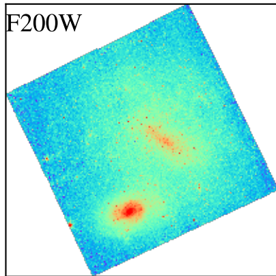
NGC4496A
