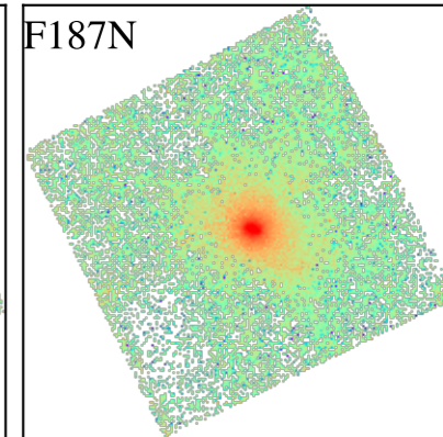
NGC4457
