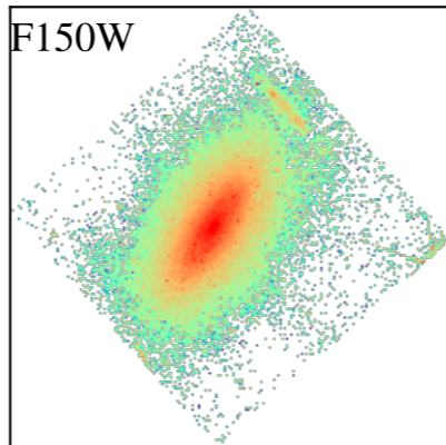
NGC1546
