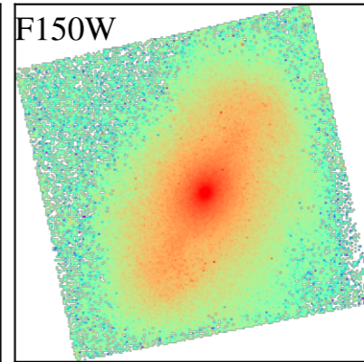
NGC5134
