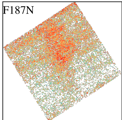
NGC7456
