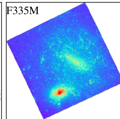
NGC4496A
