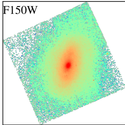
NGC3626
