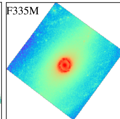
NGC1097
