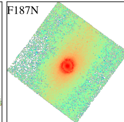
NGC1097
