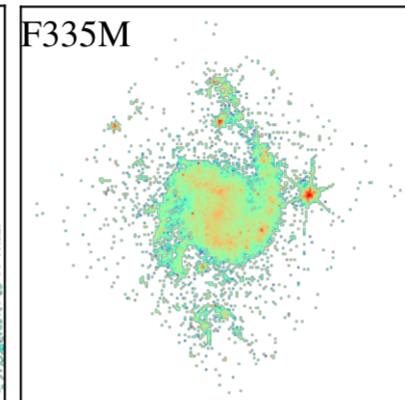
NGC2283
