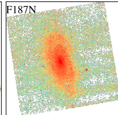
NGC2090
