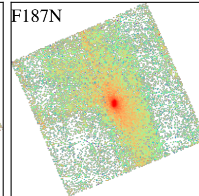
NGC4941
