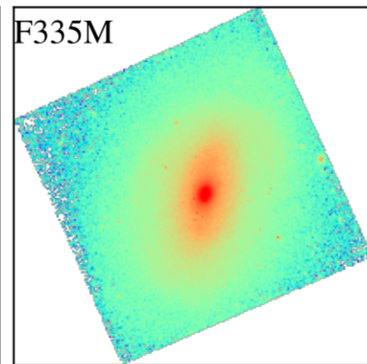
NGC3626
