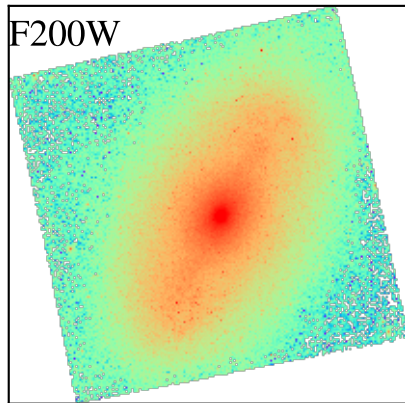
NGC5134
