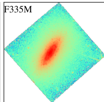
NGC1546
