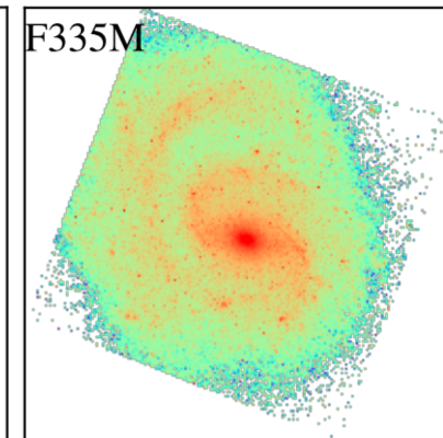
NGC1637
