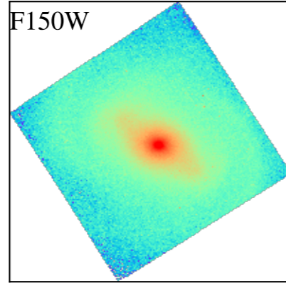
NGC4579
