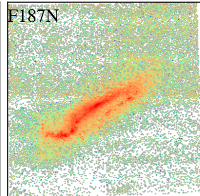
NGC1511
