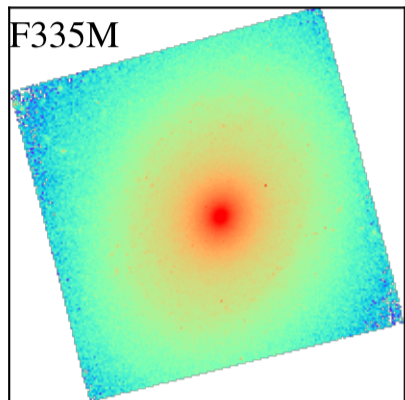
NGC2775
