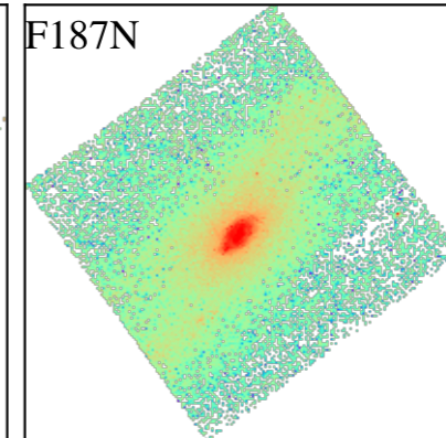
NGC1808
