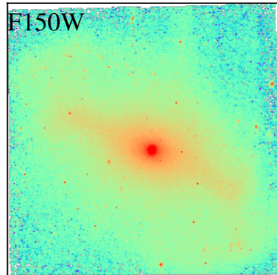
NGC2566
