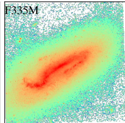
NGC1511
