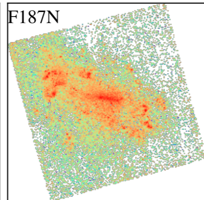
NGC1559
