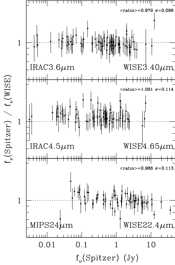
Figure 7. Comparison of Spitzer - and aperture-based global photometry with total WISE photometry.
