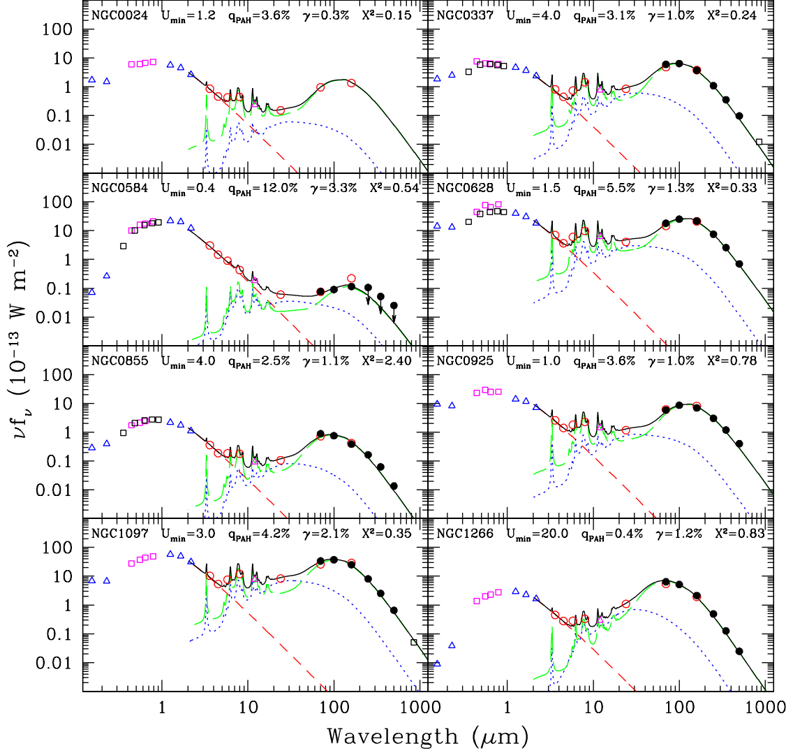
Figure 4. Globally-integrated infrared/sub-millimeter spectral energy distributions for all the galaxies in the KINGFISH sample, sorted by Right Ascension. The following symbols are utilized: filled circles ( Herschel ), triangles ( GALEX , 2MASS , and WISE ), open circles ( Spitzer ), squares ( BVR CIC and ugriz and SCUBA ). Arrows indicate 5\sigma upper limits (and lower limits in the case of NGC 3034). The solid curve is the sum of a 5000 K stellar blackbody (short dashed) along with models of dust emission from PDRs (dotted; U > U_{\min} ) and the diffuse interstellar medium (long dashed; U = U_{\min} ). The fitted parameters from these Draine & Li (2007) model fits are listed within each panel along with the reduced \chi^2 (see § 4.2 for details). While the plotted data are corrected for Galactic extinction, the fluxes tabulated in Table 3 are not corrected.
