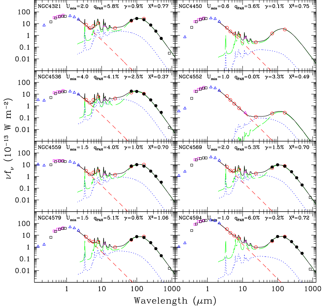
Figure 4. Globally-integrated infrared/sub-millimeter spectral energy distributions for the KINGFISH sample (continued).
