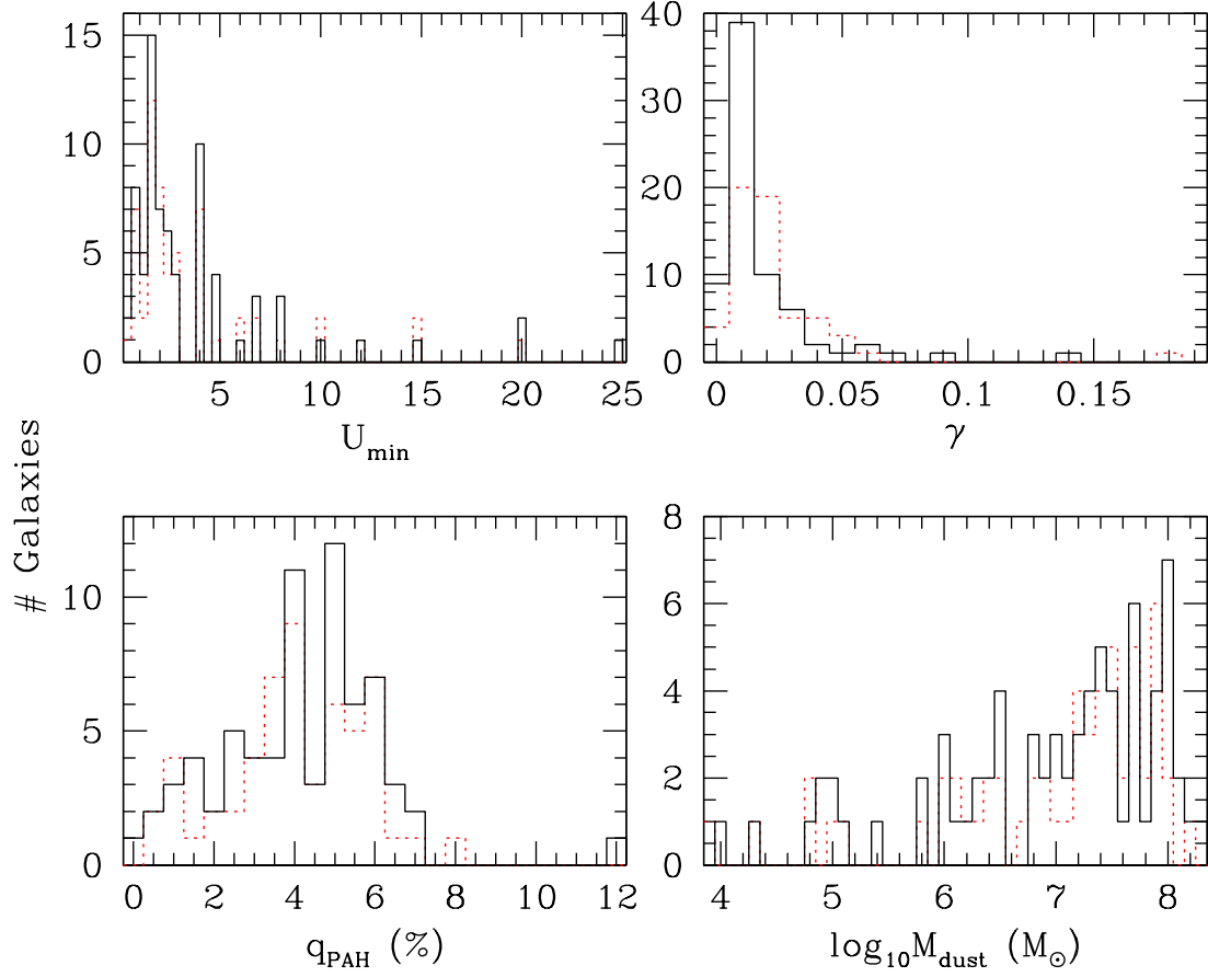
Figure 5. Comparison of DL07 output fit parameters from Dale et al. (2012) for the KINGFISH sample (red dotted line) with those measured here for the updated SINGS/KINGFISH sample (black solid line).
