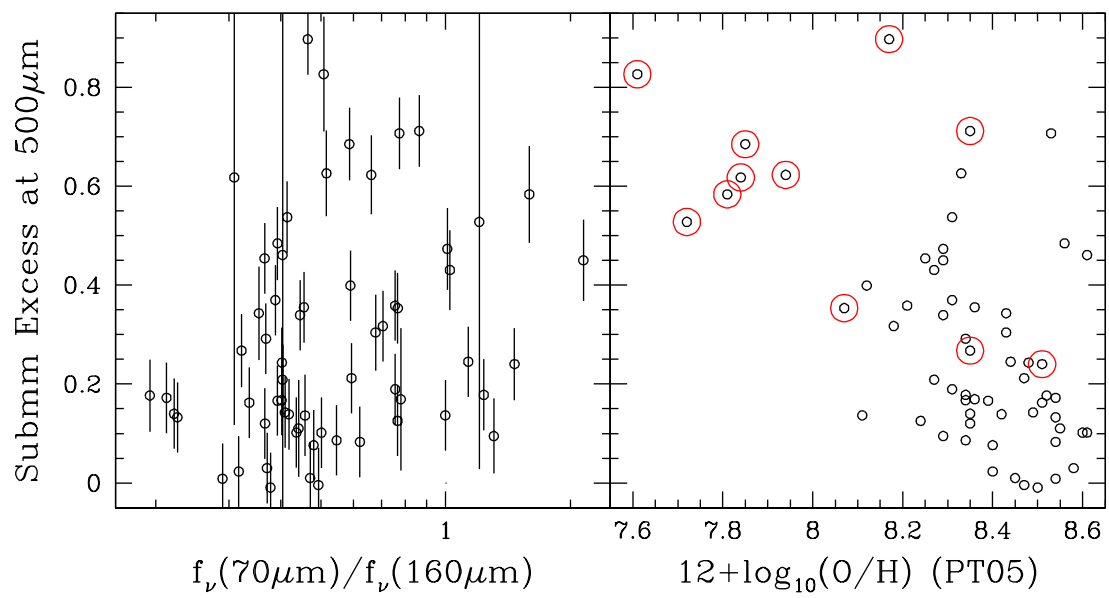
Figure 6. The submillimeter excess parameter \xi(500\mu\text{m}) (see Equation 4) as a function of far-infrared color and characteristic oxygen abundance as derived from Moustakas et al. (2010). Red circles indicate irregular galaxies ( T = \text{Sm, Im, or I0} ).
