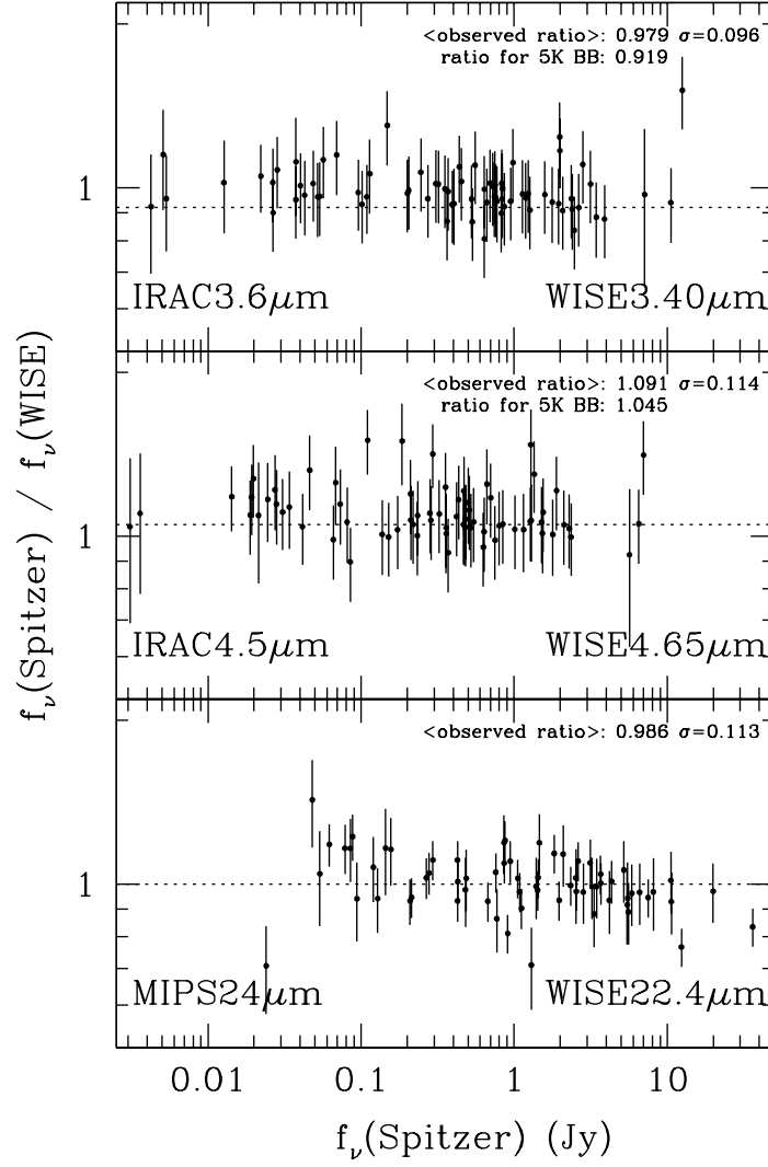
Figure 7. Comparison of Spitzer - and aperture-based global photometry with total WISE photometry. The dotted lines for the top two panels indicate the expected flux density ratios for a 5000 K blackbody.
