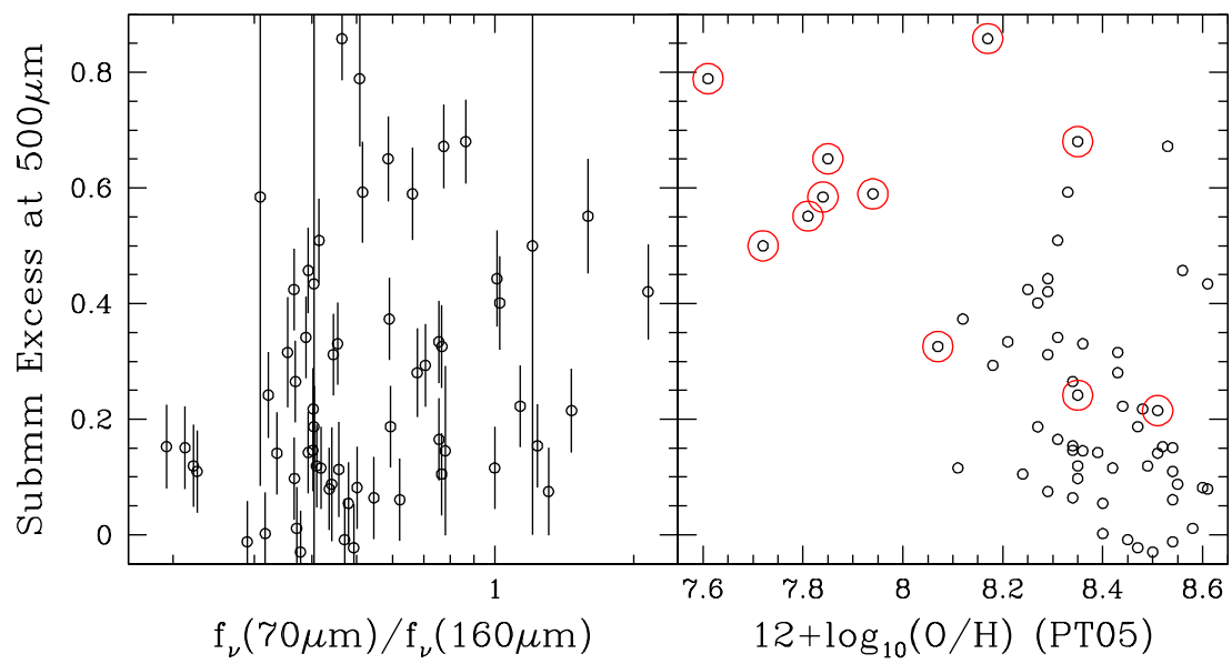
Figure 6. The submillimeter excess parameter \xi(500\mu\text{m}) (see Equation 6) as a function of far-infrared color and characteristic oxygen abundance as derived from Moustakas et al. (2010). Red circles indicate irregular galaxies ( T = \text{Sm, Im, or I0} ).
