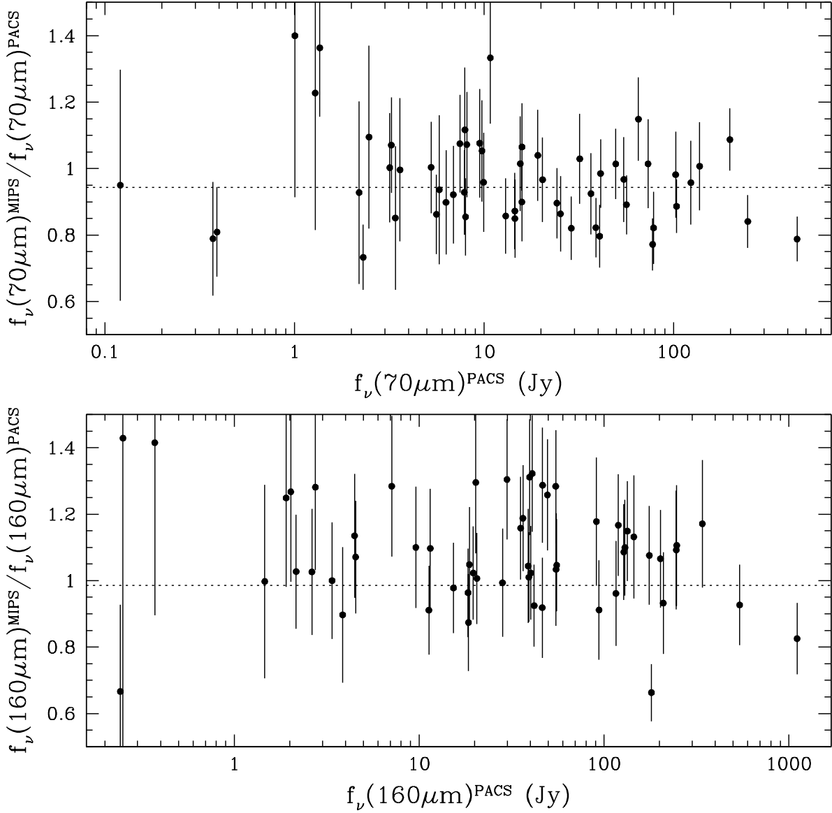
Fig. 2.— A comparison of spatially-integrated Spitzer/MIPS and Herschel/PACS photometry at 70\ \mu\text{m} (top) and 160\ \mu\text{m} (bottom) for all sample galaxies. The horizontal dotted lines indicate the ratios corresponding to perfect agreement between data taken by the two observatories, after accounting for differences in the Spitzer and Herschel spectral responses and calibration schemes; for typical galaxy spectral energy distributions, the dotted lines differ from unity by a factor of 1.06 and 1.015 for the 70 and 160\ \mu\text{m} comparisons, respectively.
