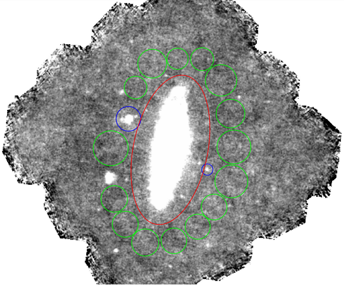
Fig. 1.— A PACS 160\ \mu\text{m} image of KINGFISH galaxy NGC 7331. The large red ellipse indicates the photometric aperture listed in Table 1, the green circles show the sky apertures, and the two blue circles identify sources to be removed before the photometry is executed. North is up, East is to the left.
