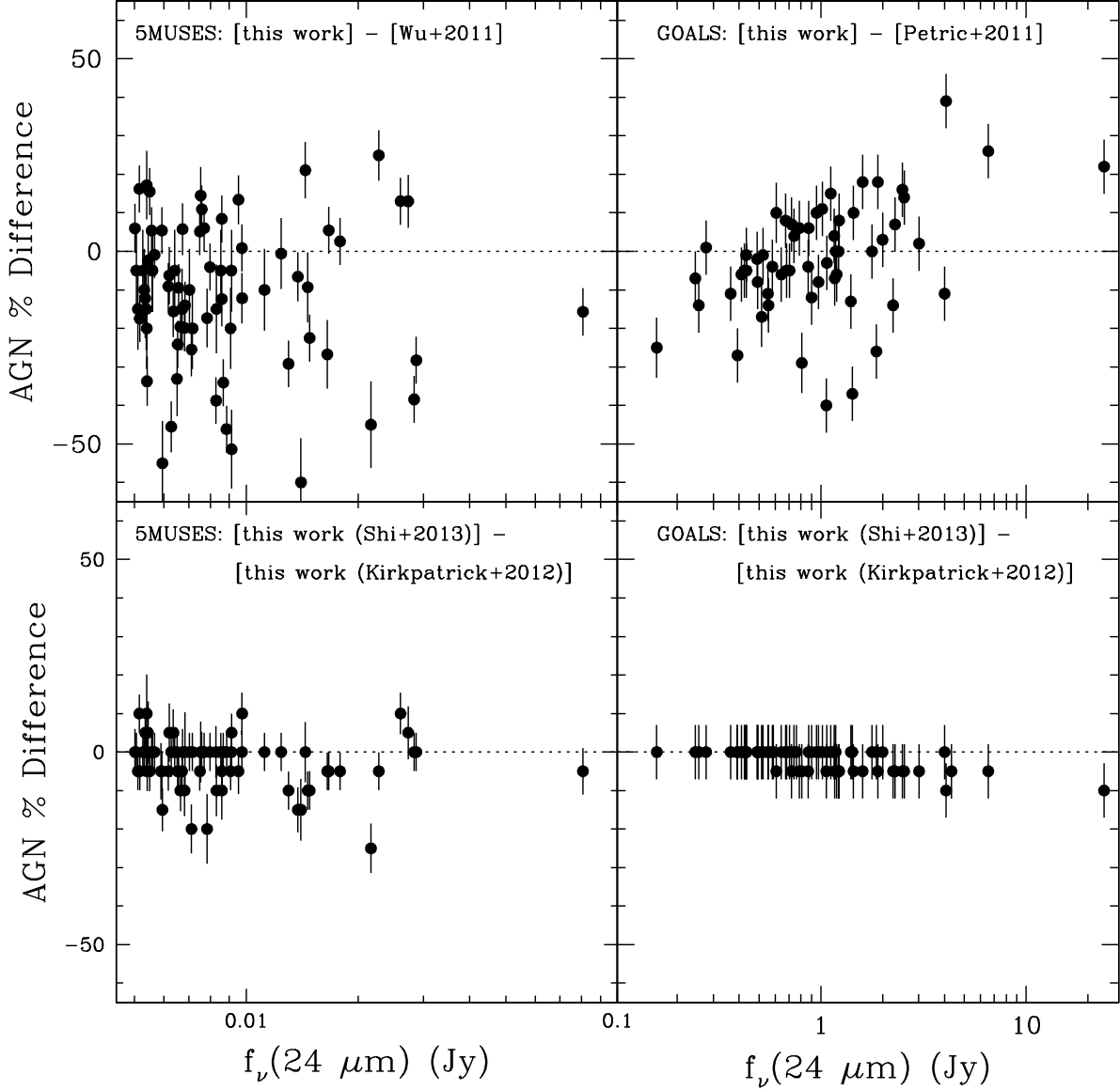
Fig. 9.— Comparisons of our mid-infrared AGN percentages using our 5.8–160 \mu\text{m} broadband SED-fitting approach and the Shi et al. (2013) quasar template with respect to those from: ( top left ) the 5–35 \mu\text{m} continuum analysis of Wu et al. (2011); ( top right ) the EW(6.2 \mu\text{m} ) + 6–15 \mu\text{m} continuum analysis of Petric et al. (2011); ( bottom ) using our broadband SED-fitting approach coupled with the Kirkpatrick et al. (2012) AGN template. The error bars displayed in the top row derive from a sum in quadrature of the standard deviations in the Monte Carlo simulations described in § 4.3 and the uncertainties from the literature fractional values (a 5% uncertainty is assumed for Wu et al. (2011)). The error bars displayed in the bottom row derive from a sum in quadrature of the standard deviations in the Monte Carlo simulations for both sets of fits.
