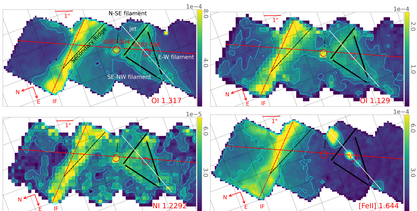
Fig. 8. Maps of O I 1.317 \mu\text{m} , 1.129 \mu\text{m} (top) as well as N I 1.2292 \mu\text{m} and [Fe II] 1.644 \mu\text{m} (bottom) across part of the NIRSpec mosaic (see the O I 1.317 \mu\text{m} and [Fe II] 1.644 \mu\text{m} maps in Fig. 7 for the full mosaic). Similar filamentary structure beyond the IF is seen in the three fluorescent lines but not in the [Fe II] 1.644 \mu\text{m} line. We set the colour range from the bottom 0.5 % to the top 99.5 % intensity levels of the data for each map (across the entire NIRSpec mosaic), excluding values of zero, edge pixels, and the two proplyds. White pixels inside the mosaic indicate values of zero reflecting issues with the data. The nearly horizontal red line indicates the NIRSpec cut and the nearly vertical red line indicates the IF. The two proplyds are indicated by the circles (left panel), the jet associated with proplyd 203-504 by a gold line and the filaments by red lines. Contours show the 77.9, 90.2, and 96 % intensity levels of the data for O I 1.317 \mu\text{m} , 70, 85, and 97 % intensity levels for O I 1.129 \mu\text{m} and 55, 81, and 96 % intensity levels for N I 1.2292 \mu\text{m} , and 80, 90.2, and 96 % intensity levels of the data for [Fe II] 1.644 \mu\text{m} (across the entire NIRSpec mosaic).
