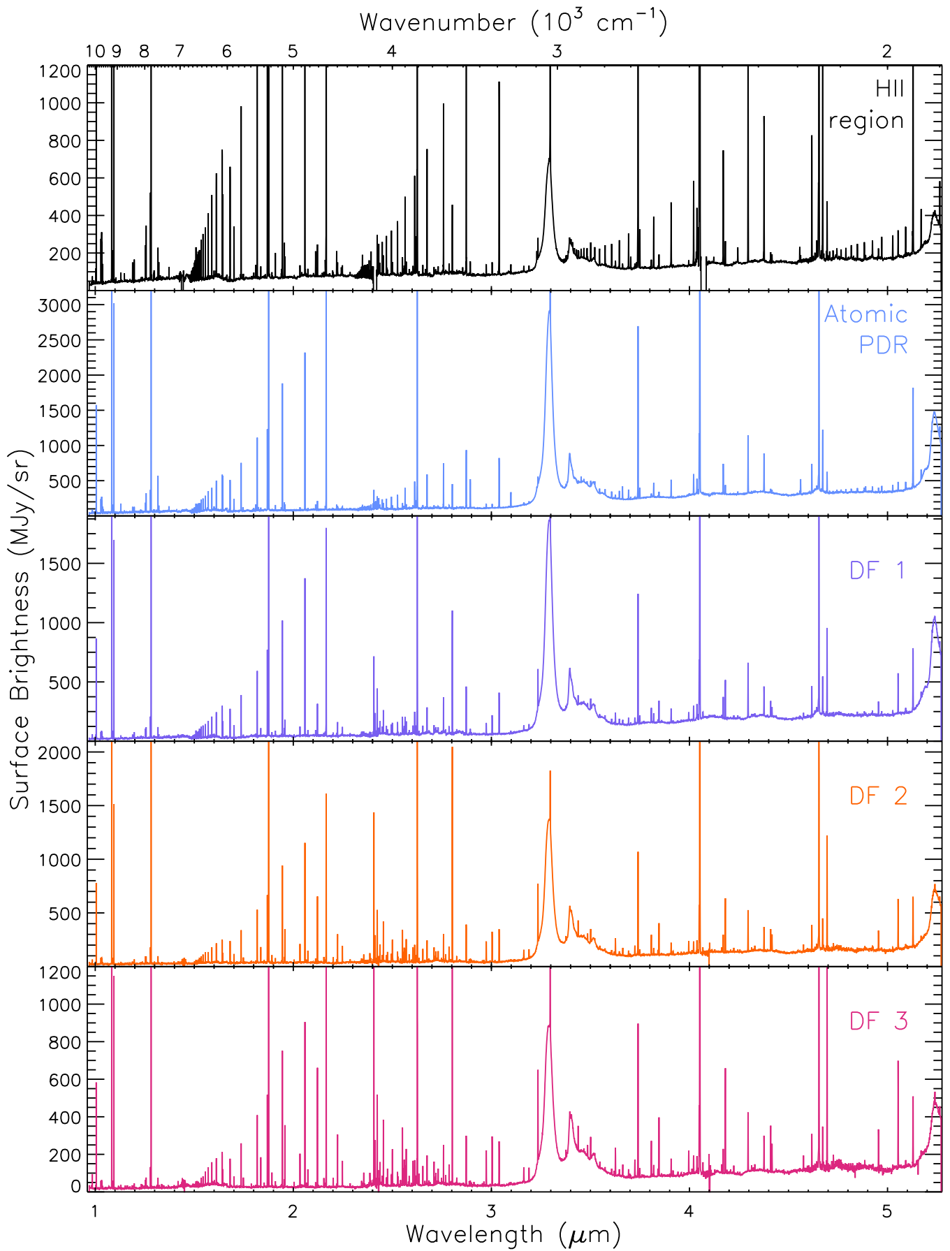
Fig. 2. Template spectra representing from top to bottom the H II region, the atomic PDR, and the dissociation fronts DF 1, DF 2, and DF 3.
